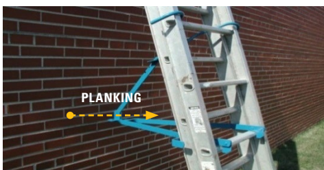
Side Rail Ladder Jack
